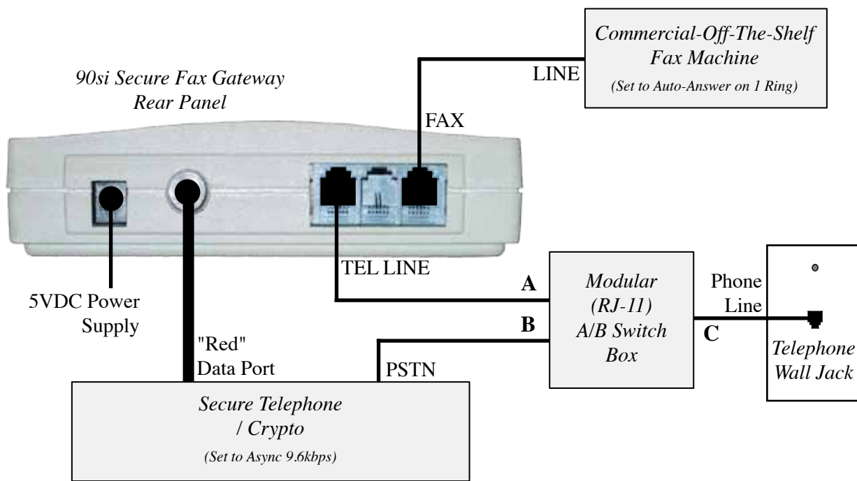
Figure 4: 1-Line, Dual-Mode with 910 Option Configuration
