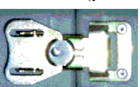
Detail of one of 6 Latches
